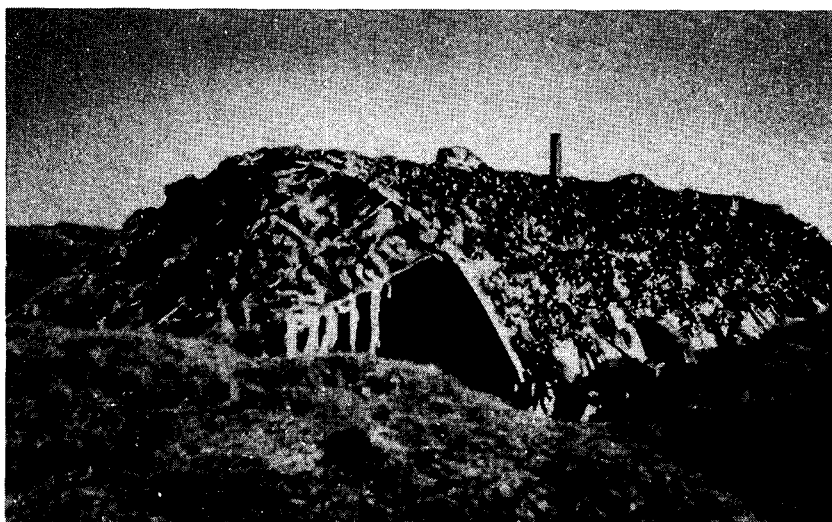
Figure 59. Here is a quonset hut blended into the terrain by a combination of digging in, texturing, and covering with a net.
