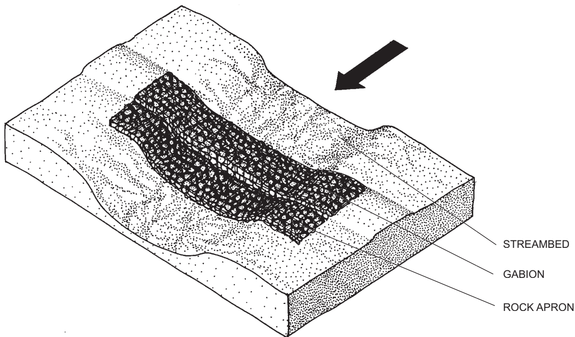
GABION IN WIDE STREAMBED
