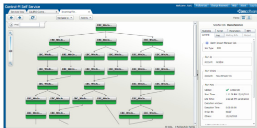
Figure 2. BMC Control-M Self Service detail view
