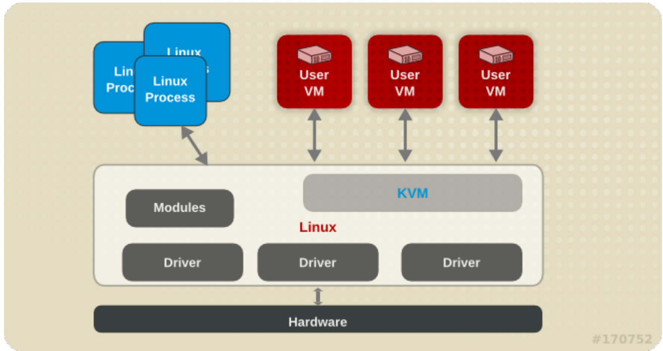
Figure 1.1. KVM architecture
