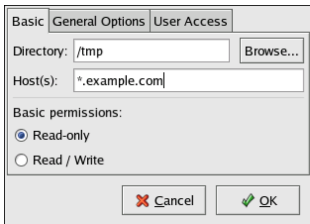
Figure 21.2. Add Share
