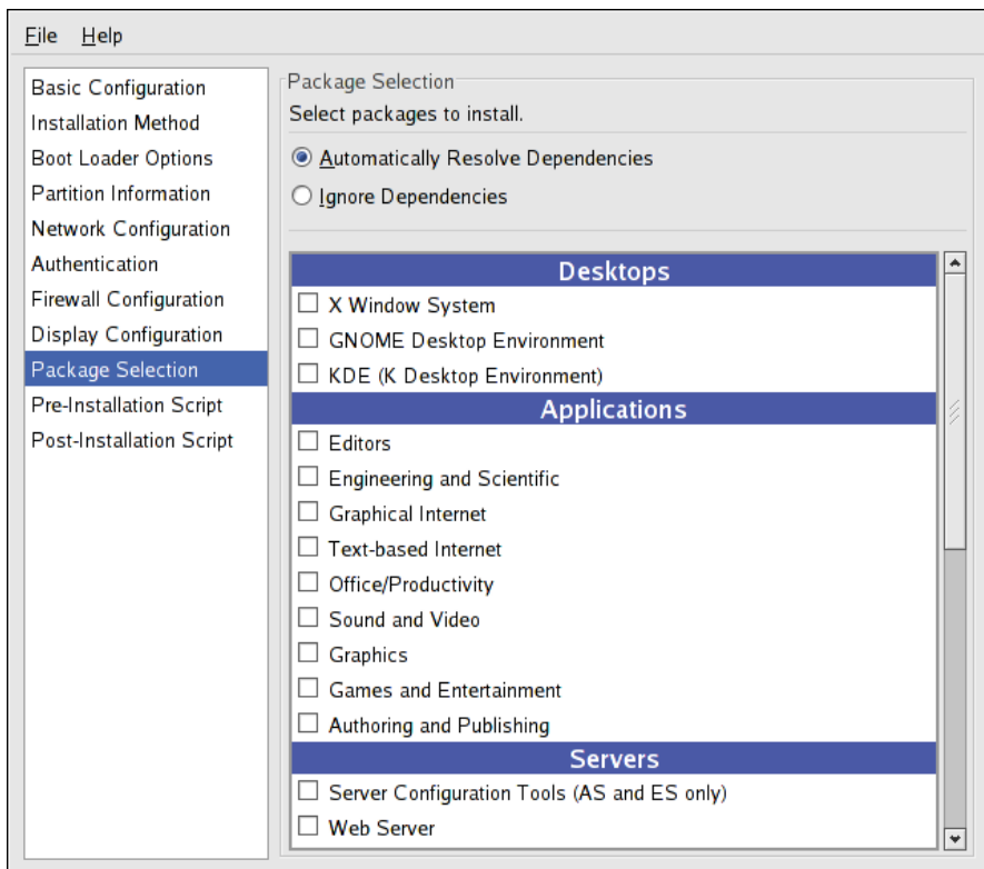
Figure 2.14. Package Selection
