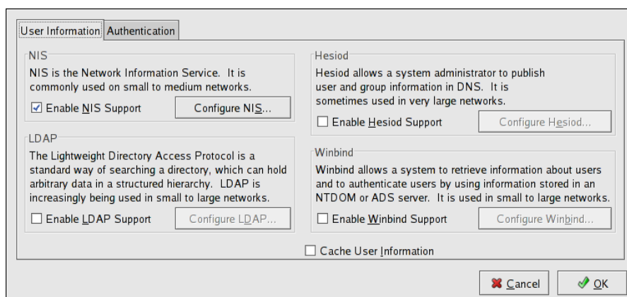
Figure 26.1. User Information
