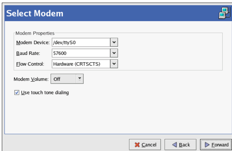
Figure 17.6. Modem Settings
