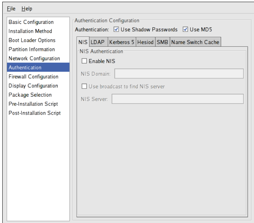
Figure 2.9. Authentication
