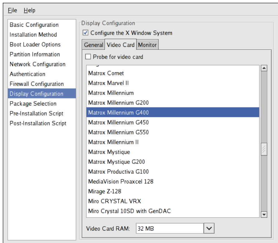
Figure 2.12. X Configuration - Video Card
