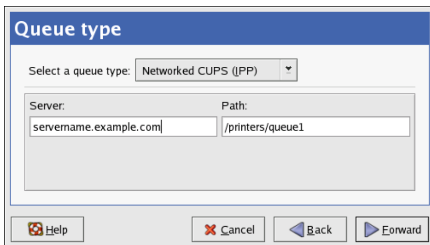
Figure 33.4. Adding an IPP Printer
