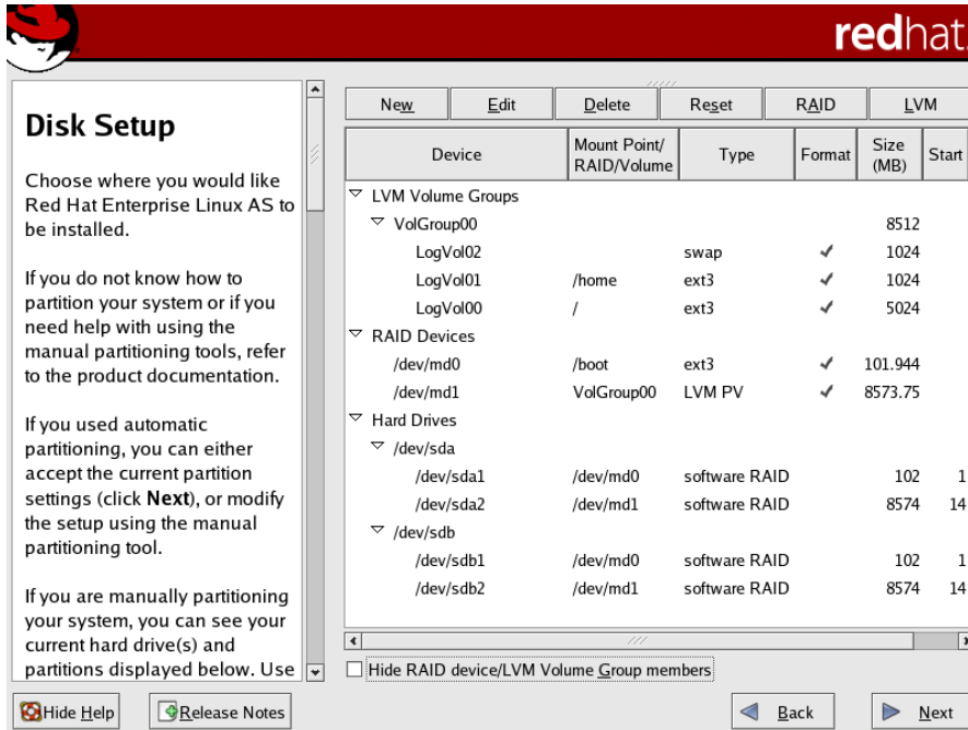
Figure 10.9. Final Sample RAID With LVM Configuration
