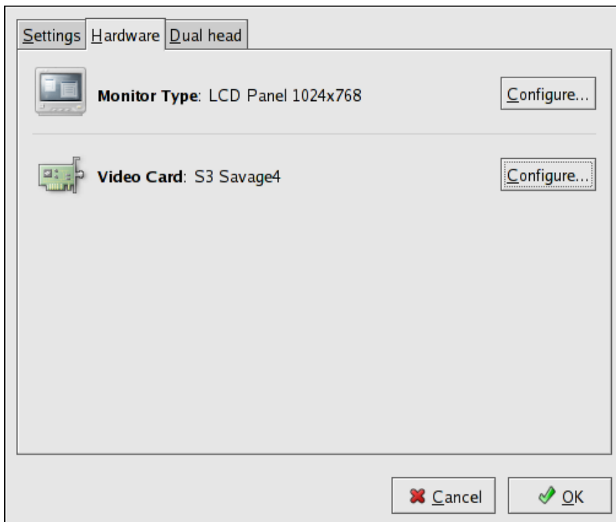
Figure 31.2. Display Hardware Settings
