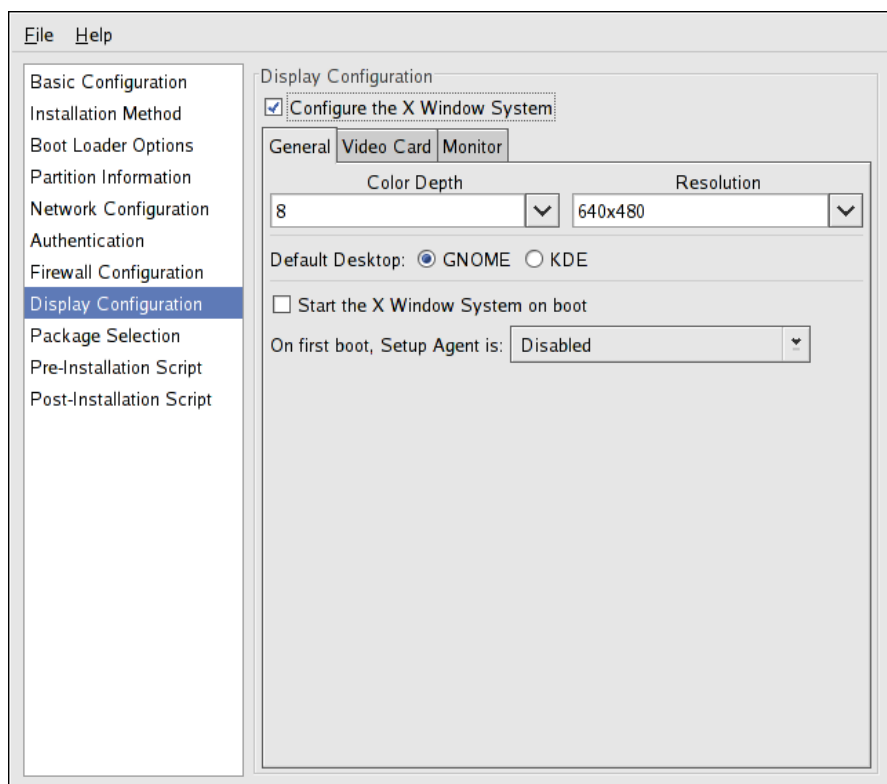
Figure 2.11. X Configuration - General
