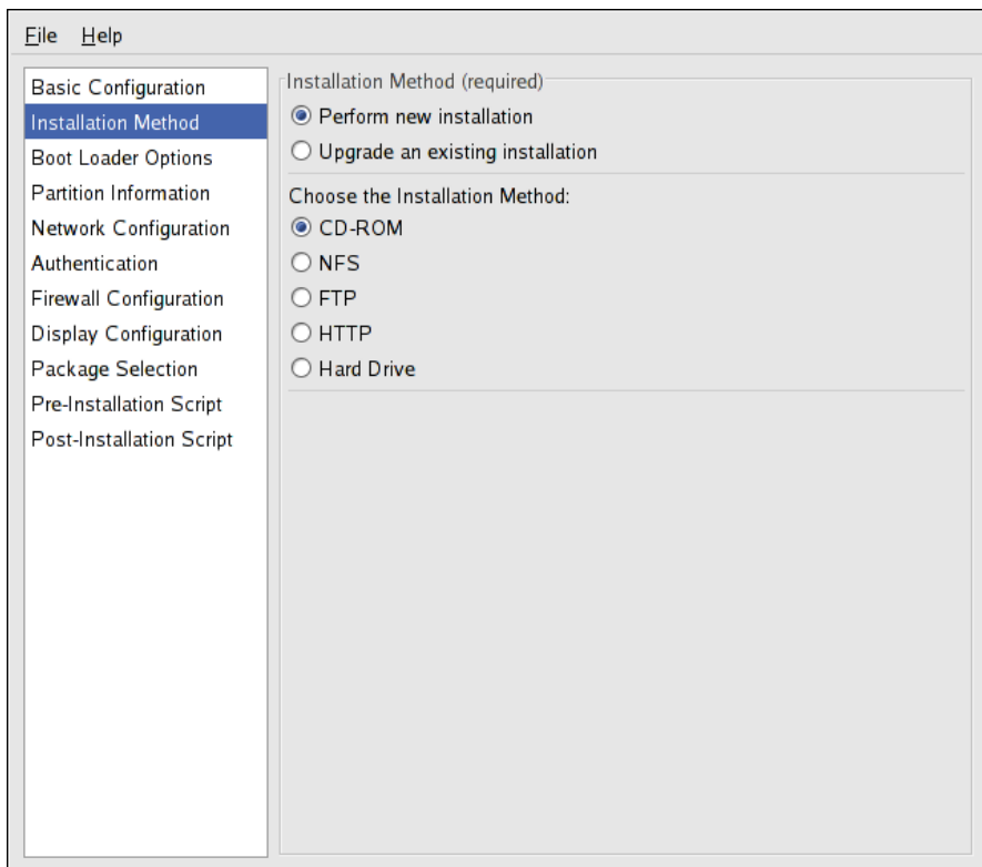
Figure 2.2. Installation Method
