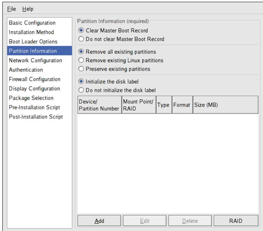
Figure 2.4. Partition Information
