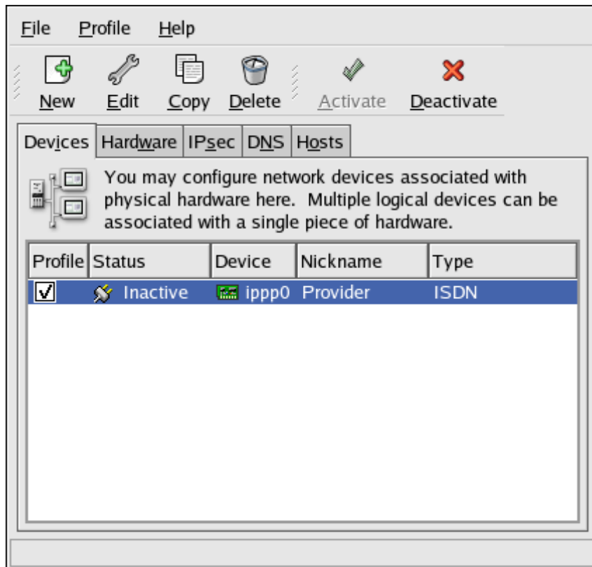
Figure 17.5. ISDN Device
