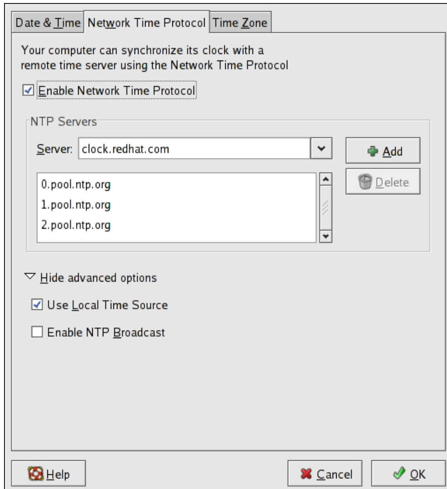
Figure 28.2. NTP Properties
