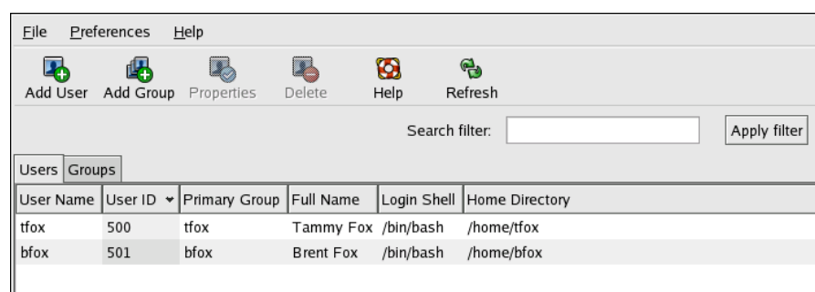
Figure 32.1. User Manager
