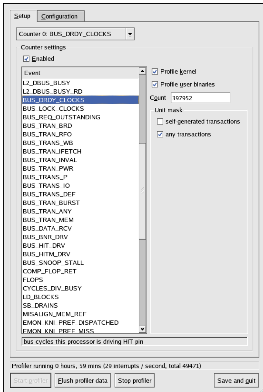
Figure 40.1. OProfile Setup
