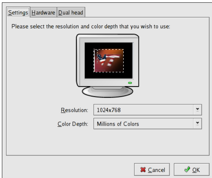
Figure 31.1. Display Settings
