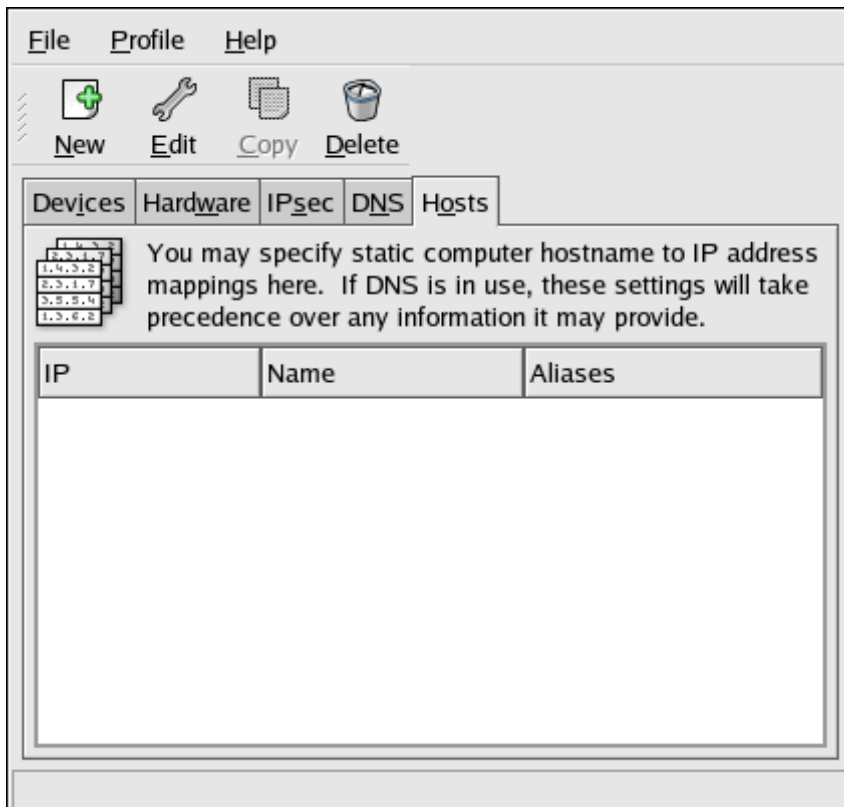
Figure 17.15. Hosts Configuration
