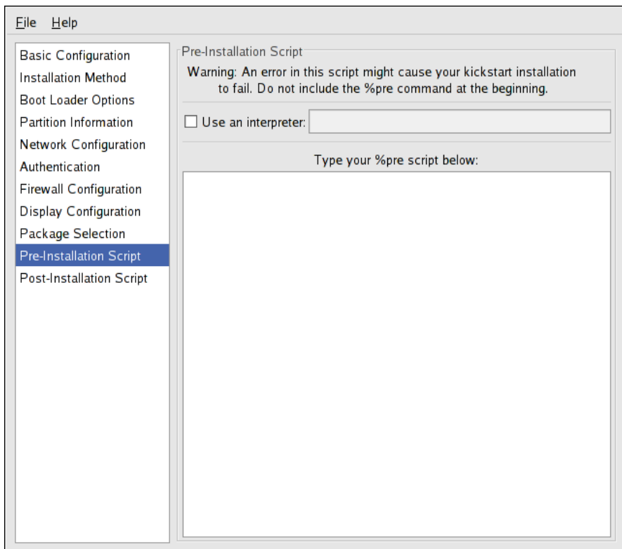
Figure 2.15. Pre-Installation Script
