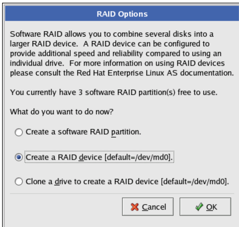
Figure 10.5. RAID Options
