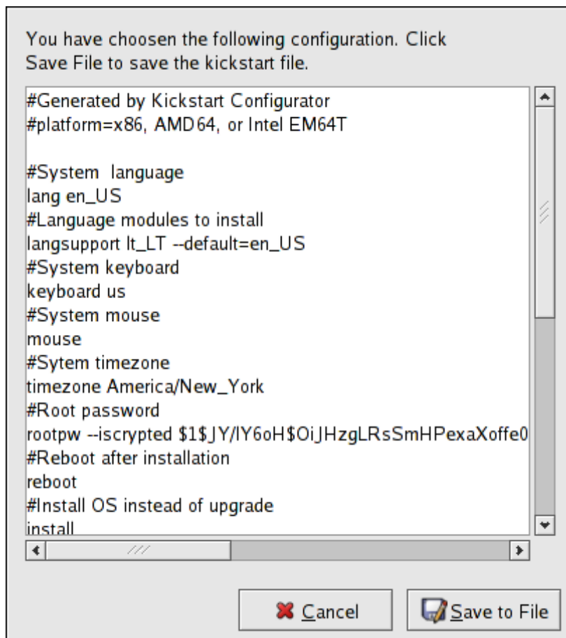
Figure 2.17. Preview
