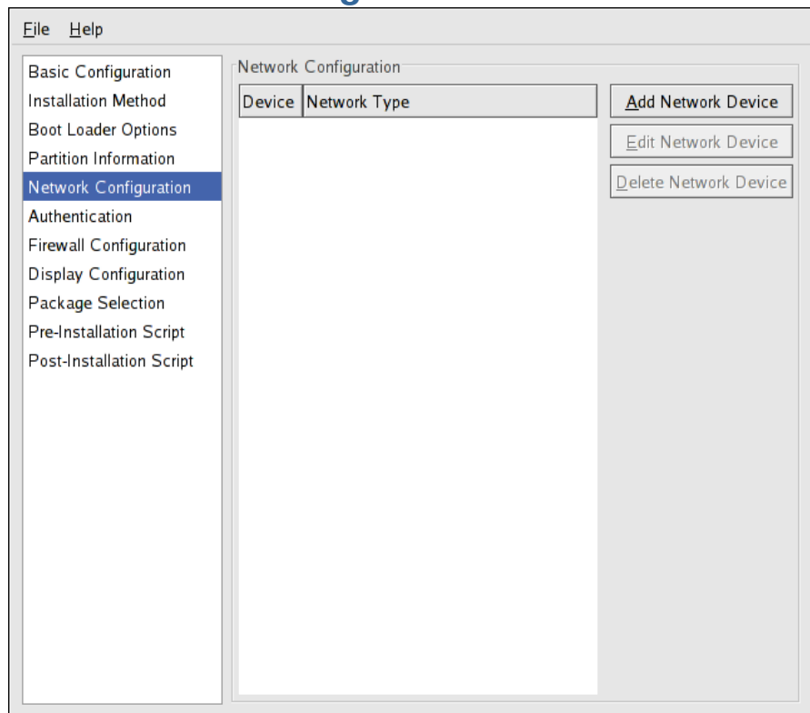
Figure 2.8. Network Configuration
