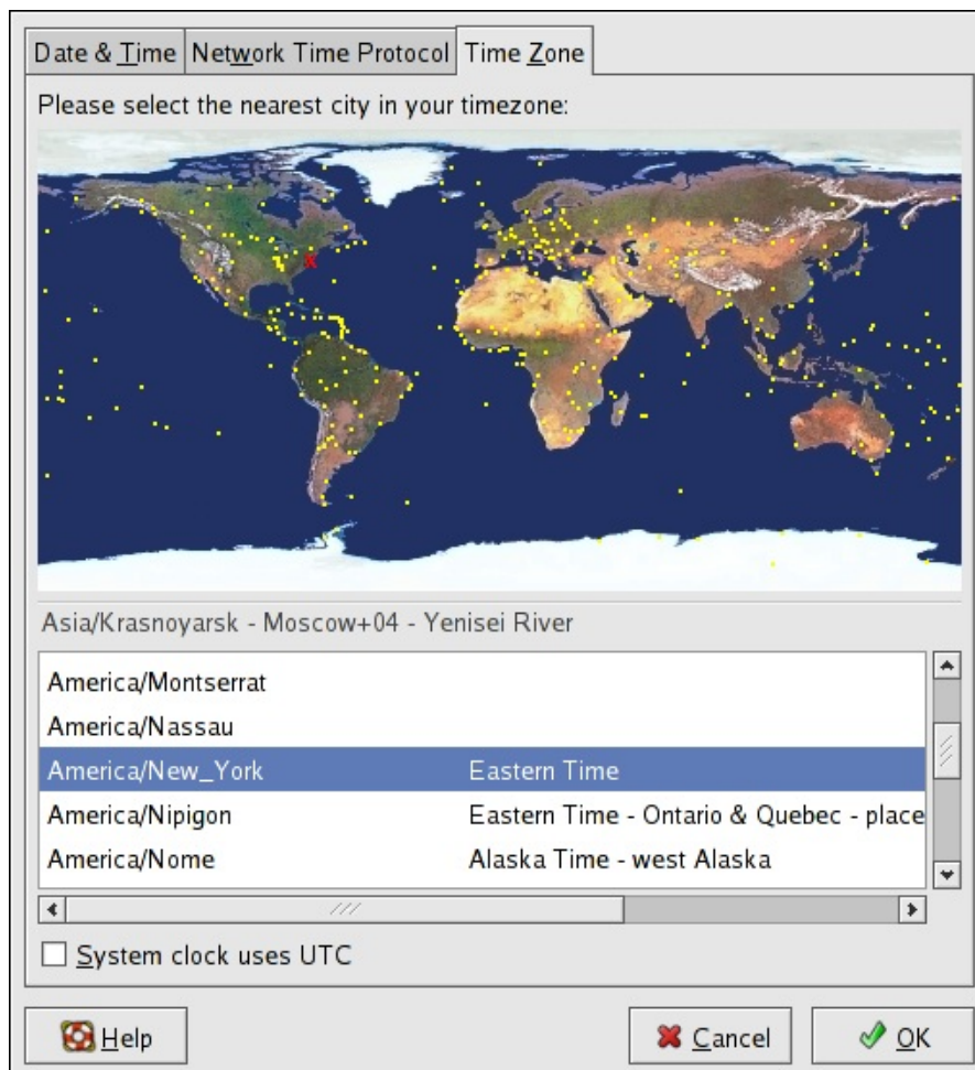
Figure 28.3. Timezone Properties
