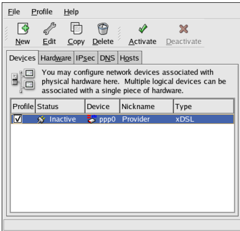
Figure 17.9. xDSL Device
