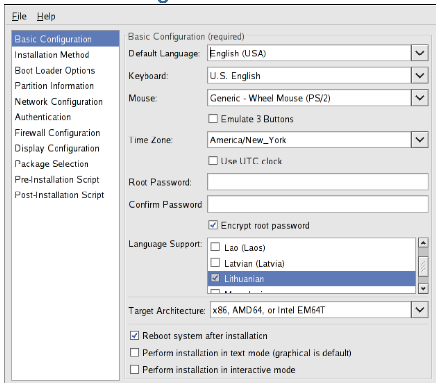
Figure 2.1. Basic Configuration
