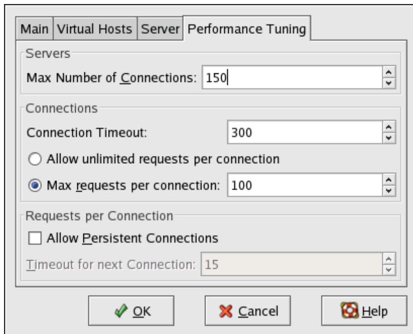
Figure 24.11. Performance Tuning
