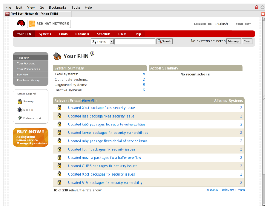
Figure 16.1. Your RHN
