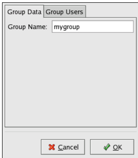
Figure 32.5. Group Properties
