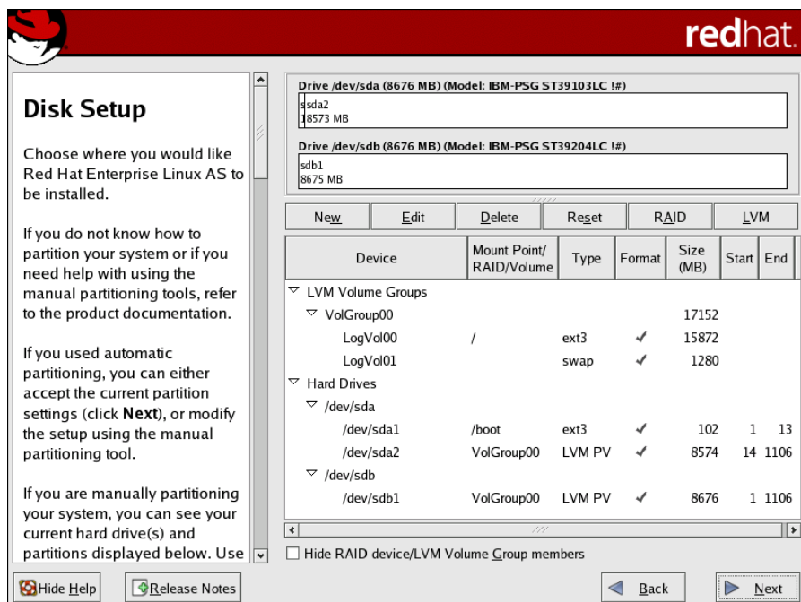
Figure 8.1. Automatic LVM Configuration With Two SCSI Drives
