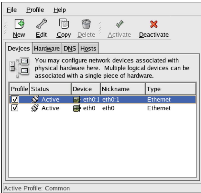
Figure 17.18. Network Device Alias Example
