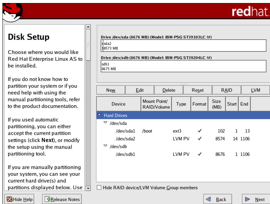
Figure 8.6. Two Physical Volumes Created
