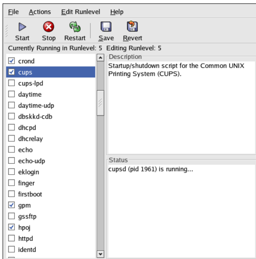
Figure 19.1. Services Configuration Tool
