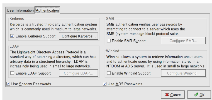
Figure 26.2. Authentication
