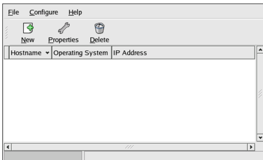
Figure 3.2. Add Hosts
