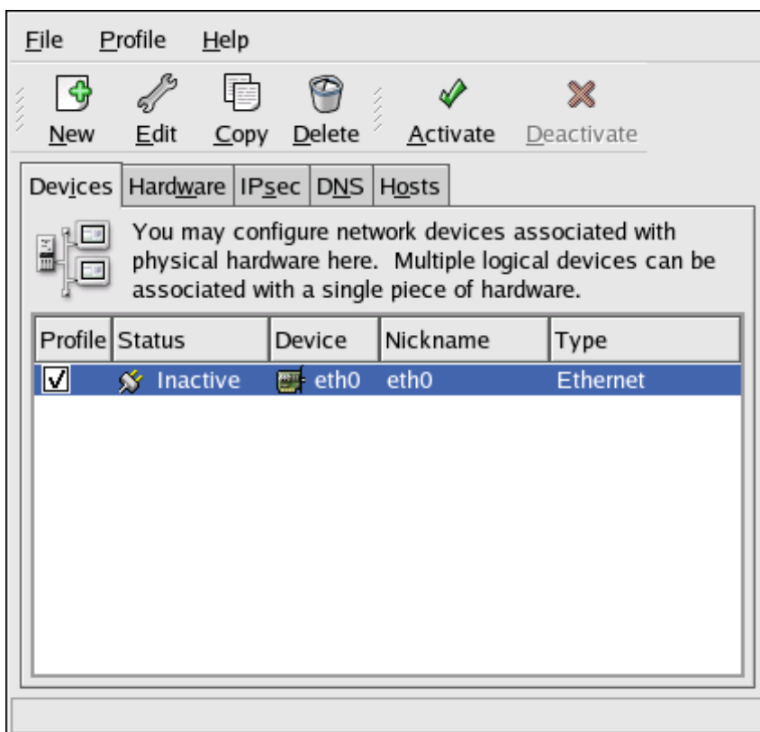
Figure 17.3. Ethernet Device
