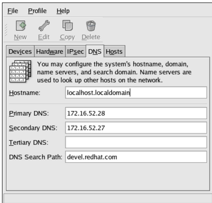
Figure 17.14. DNS Configuration
