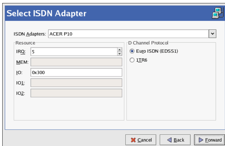
Figure 17.4. ISDN Settings
