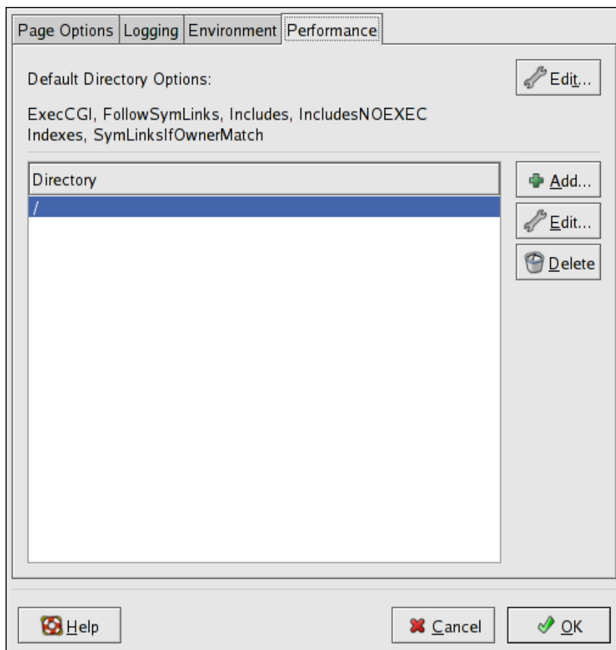
Figure 24.6. Directories
