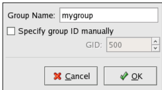
Figure 32.4. New Group
