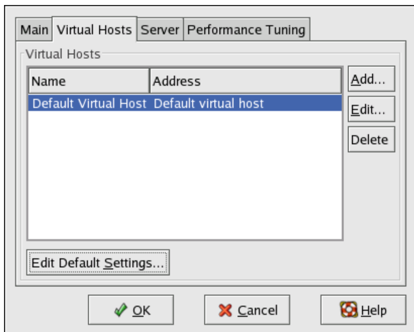
Figure 24.8. Virtual Hosts
