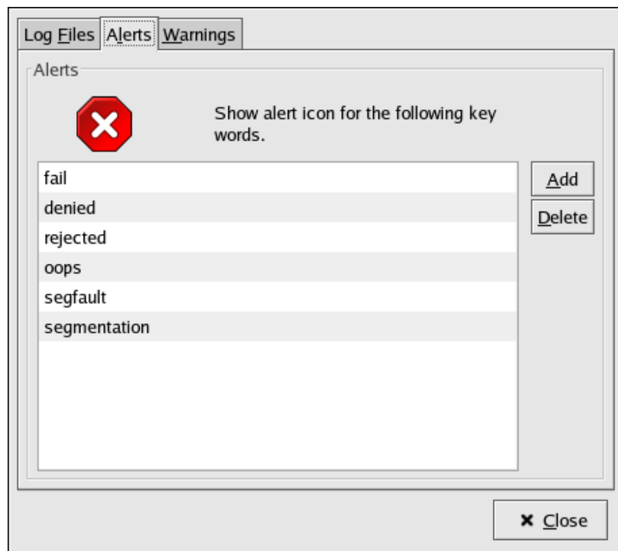
Figure 35.4. Alerts
