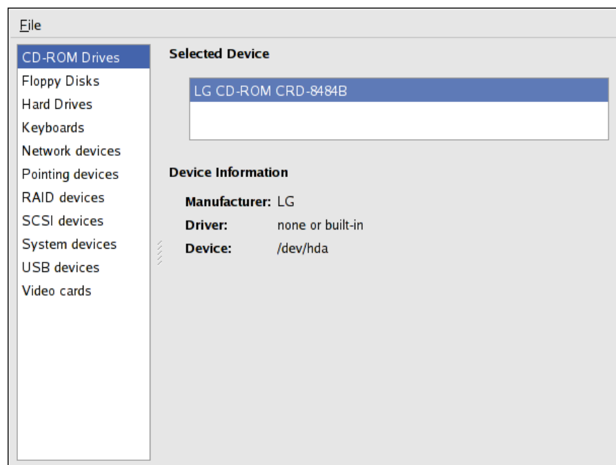
Figure 39.4. Hardware Browser
