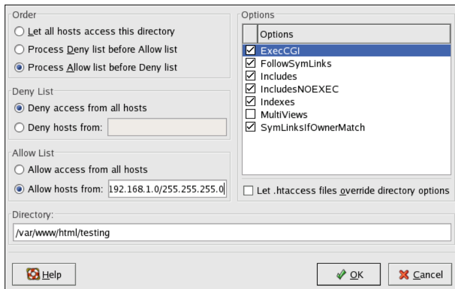
Figure 24.7. Directory Settings
