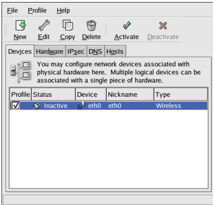
Figure 17.13. Wireless Device
