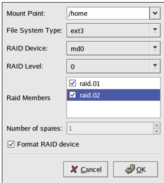
Figure 2.7. Creating a Software RAID Device
