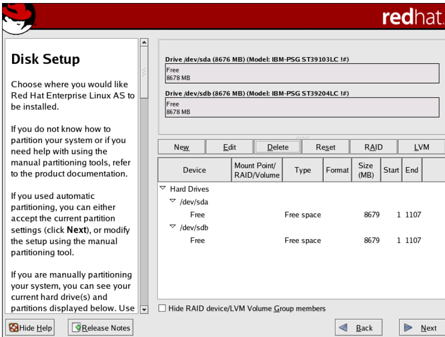
Figure 10.1. Two Blank Drives, Ready For Configuration
