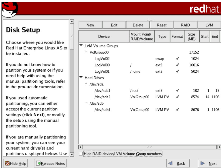
Figure 8.10. Final Manual Configuration
