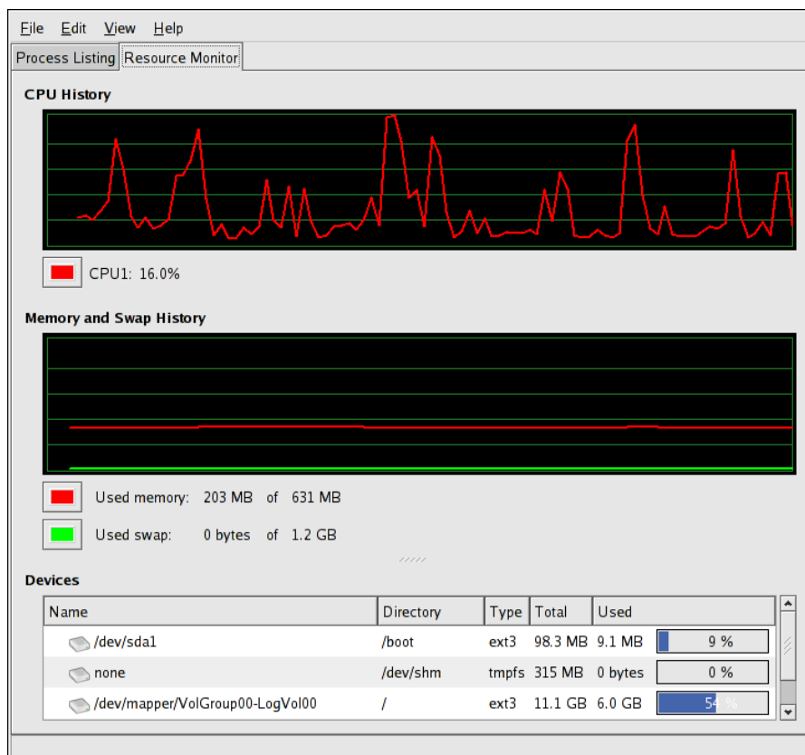
Figure 39.2. GNOME System Monitor - Resources tab
