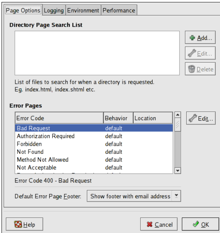
Figure 24.3. Site Configuration
