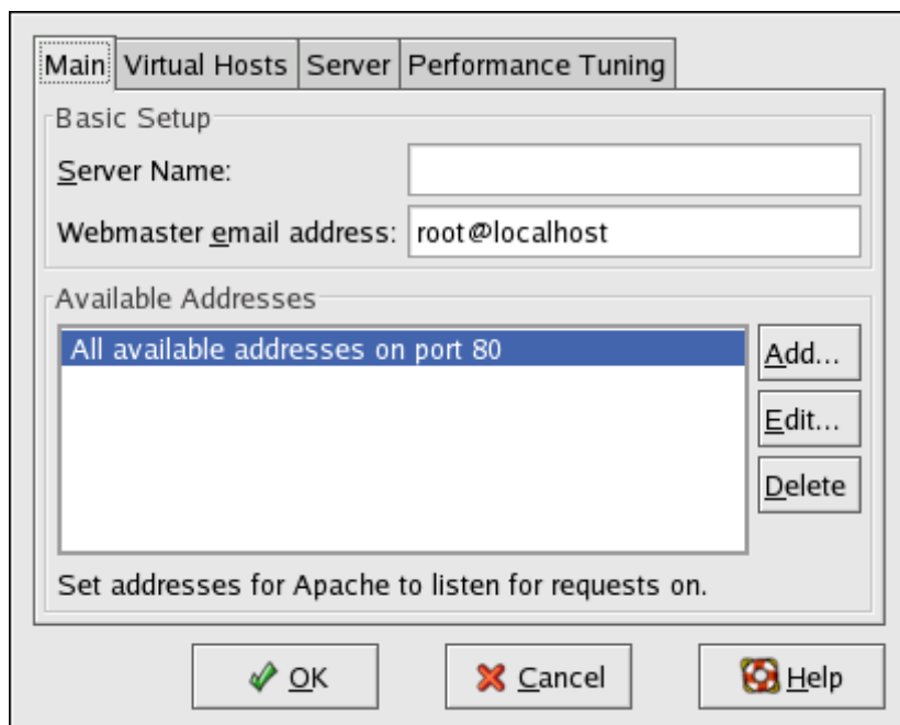
Figure 24.1. Basic Settings
