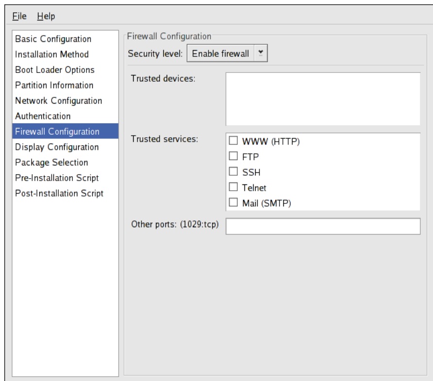
Figure 2.10. Firewall Configuration
