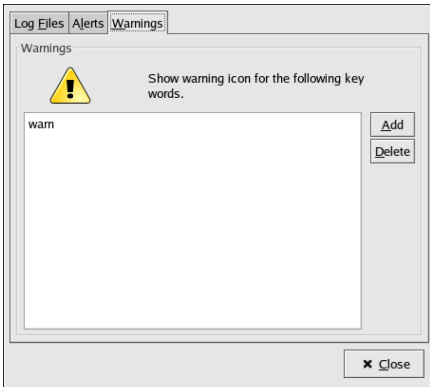
Figure 35.5. Warning
