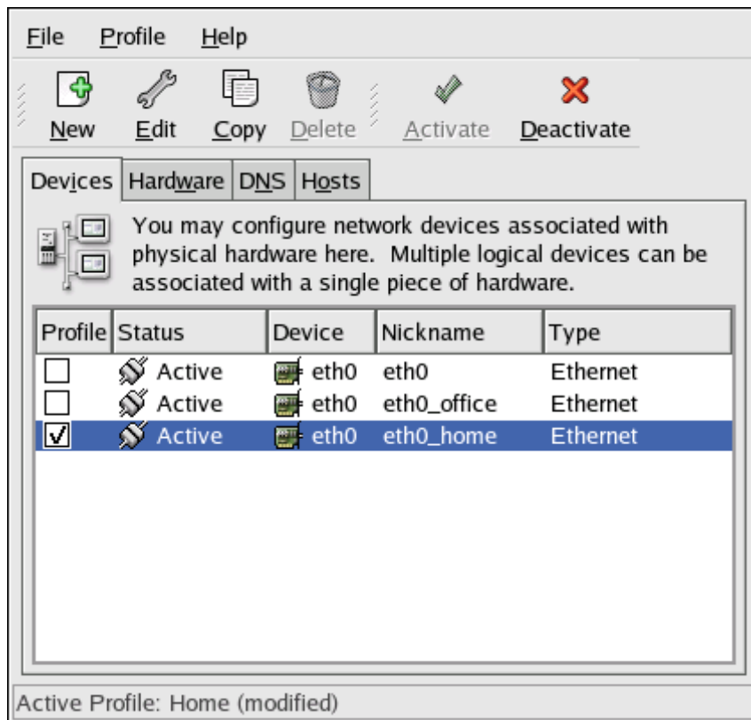
Figure 17.17. Home Profile
