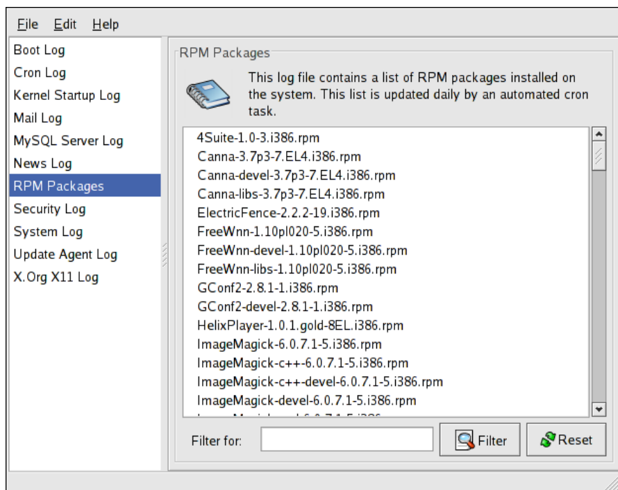
Figure 35.1. Log Viewer
