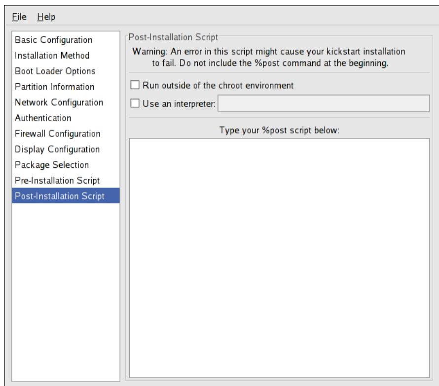
Figure 2.16. Post-Installation Script
