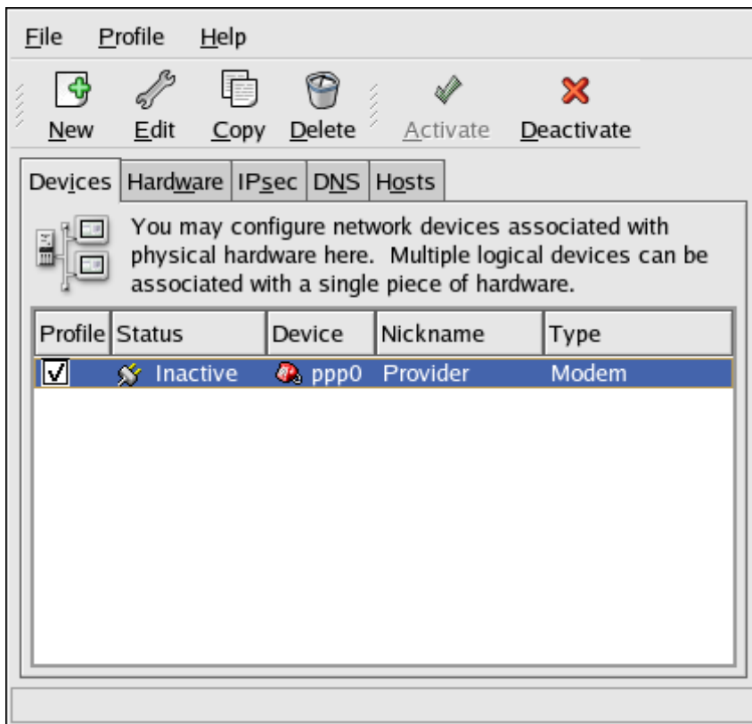
Figure 17.7. Modem Device
