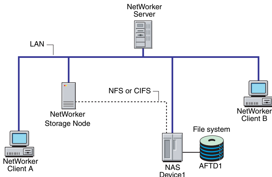
Figure 29 AFTD Configuration
