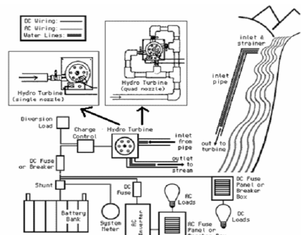
Fig. 1 Example of pico-hydro power system applications at rural area
