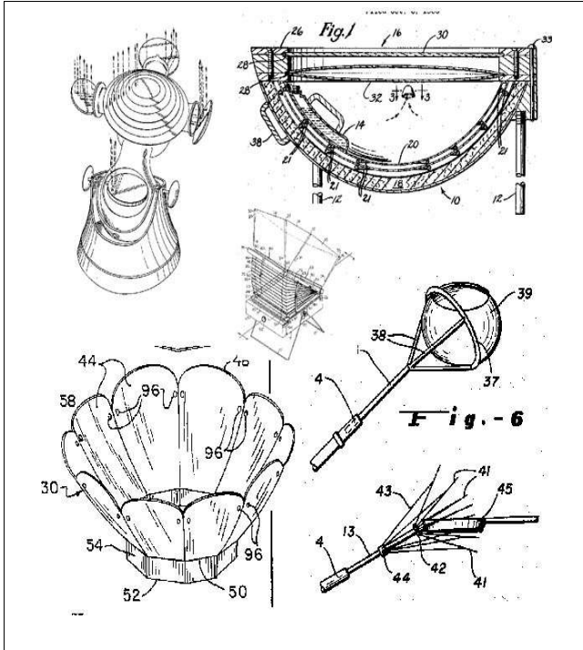
Figure 1. Drawings from different solar cooker patents.
