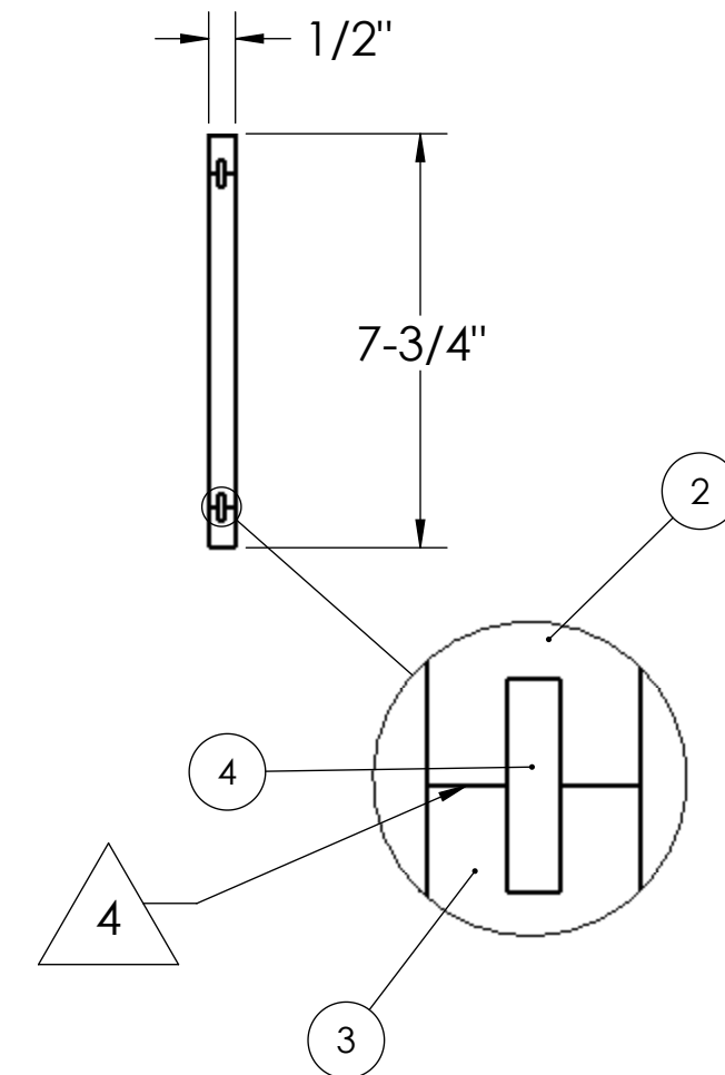
MASONITE INSERT IN PLACE 4X
