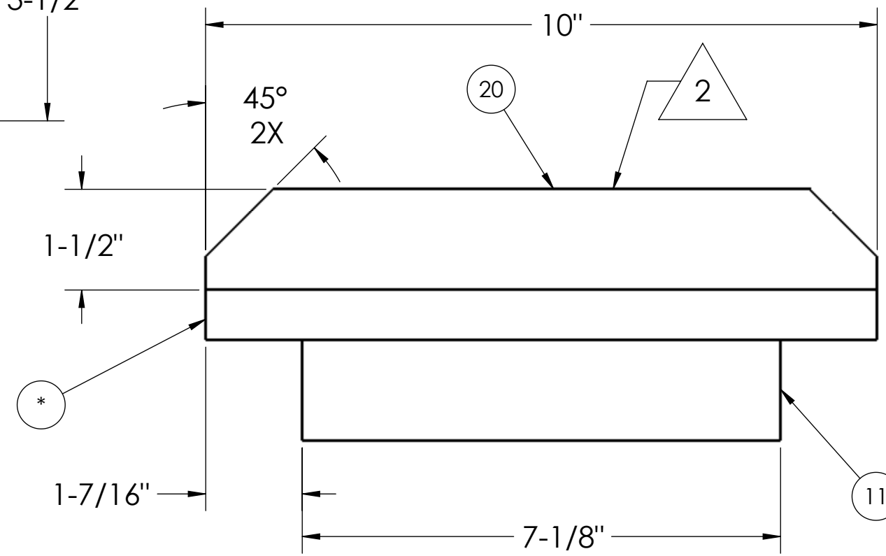
LANDING BOARD
