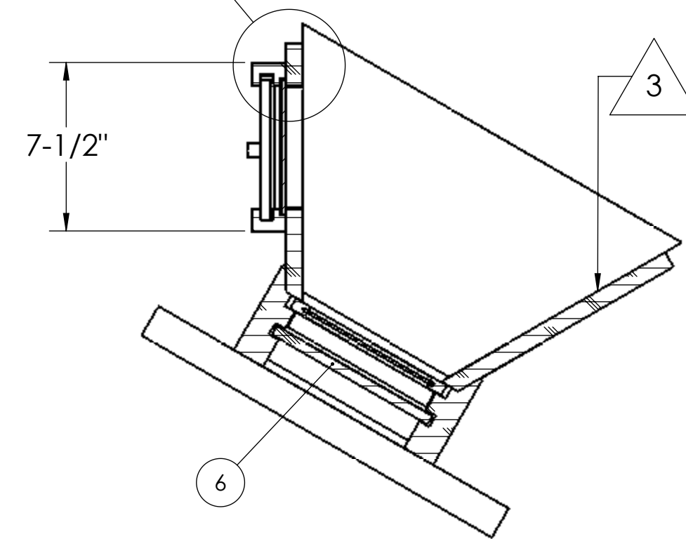
SECTION M-M
