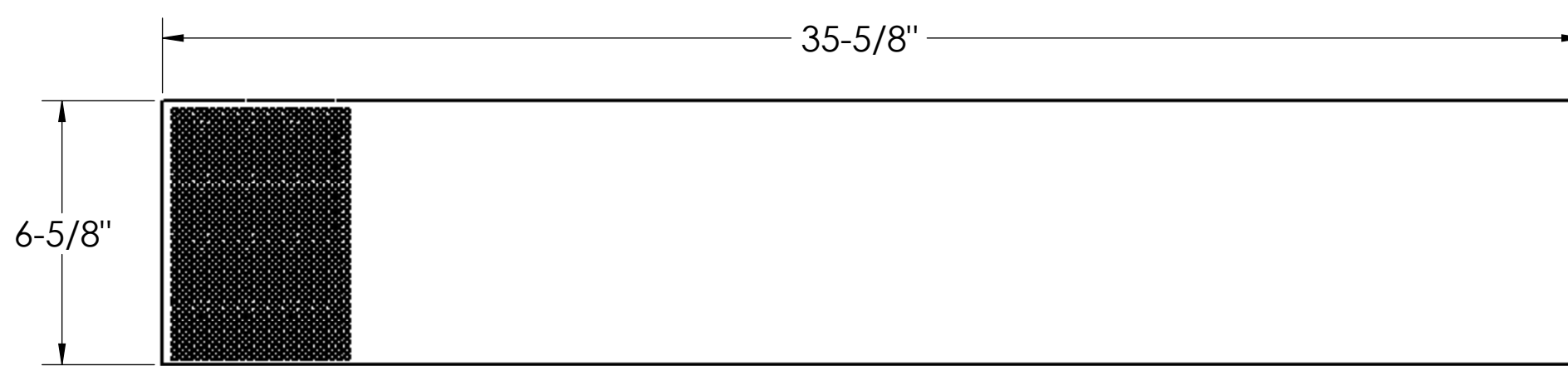
UNCOATED STEEL HARDWARE CLOTH #6 X .046" WIRE DIA
