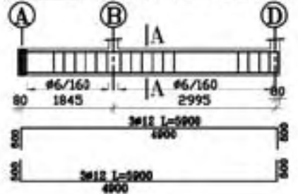
MB-1 Mat beam A-B-D on axis 1
