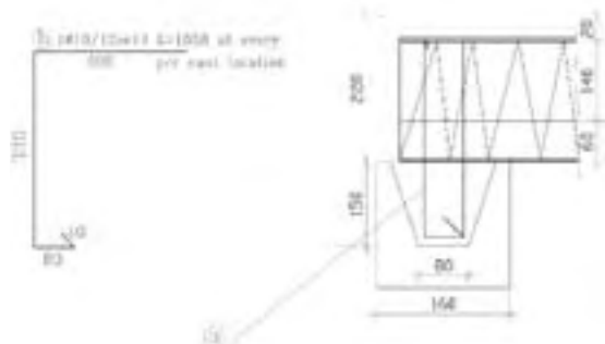
DETAIL A: Additional re-bar at edge
