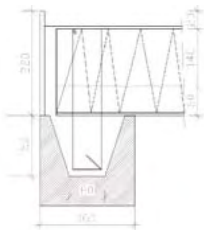
FIG-6s typical connection detail of U beam and pre cast beam
