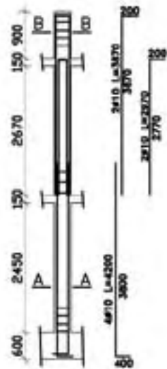
C-1 (8pcs)
