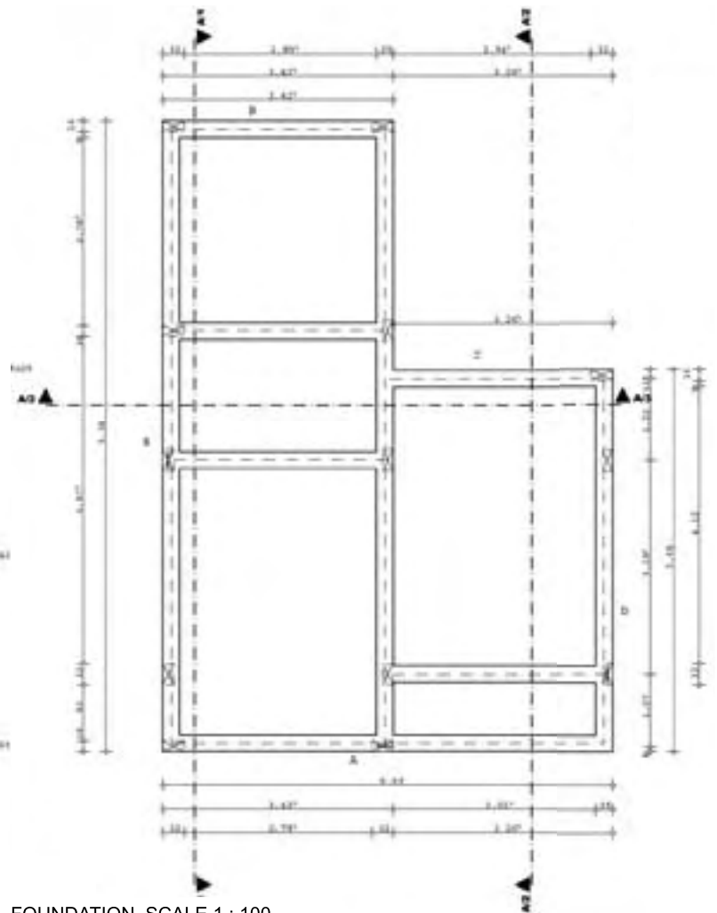
FOUNDATION, SCALE 1 : 100
