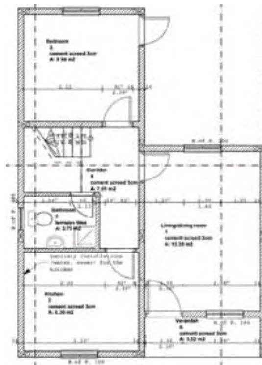
Building plan for the model
