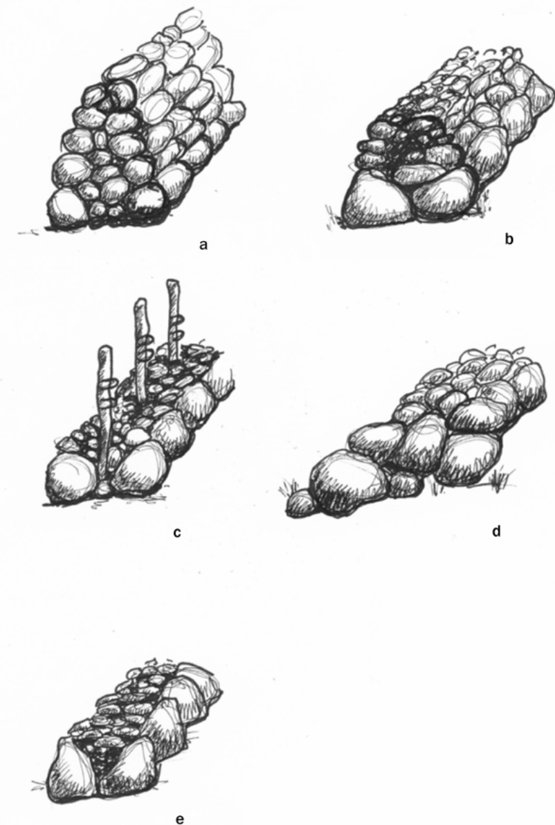
Figure 2. Five of many Estonian types of dry laid stone: (a) woods fence, meadow fence; (b) field fence, village fence; (c) sheep fence; (d) berm fence; (e) split granite fence.
