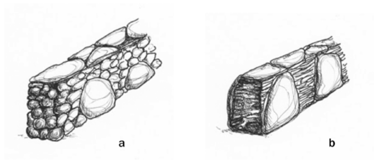
Figure 5. Mixed material walls on Gotland: (a) placing big rocks in between small ones; (b) rearing up stone slabs next to each other in two parallel rows and filling the core with smaller stones. Drawings by Elle Lepik.
