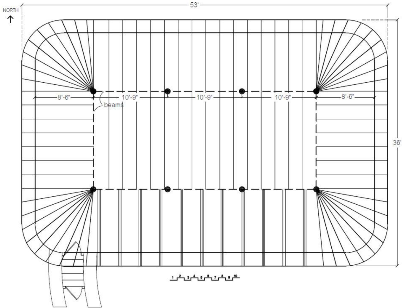
Roof Plan
