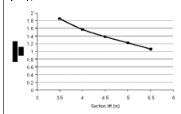
Figure 6: Pump performance data for Masvingo pump, Zimbabwe
