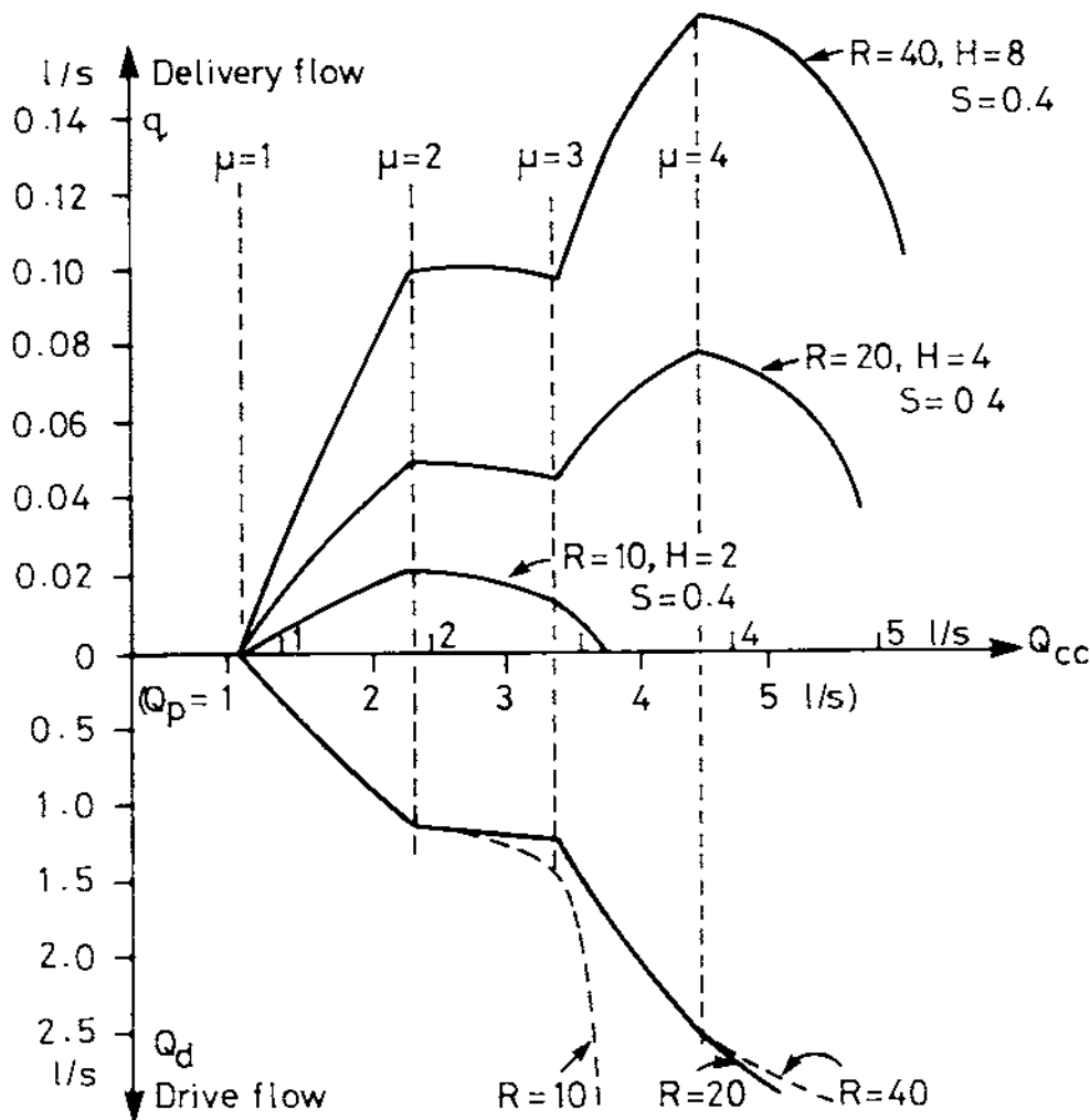
Fig. 2 Characteristic for pump type M8 with 50 mm drive pipe when tuning ( Q_{cc} ) is varied (delivery head of h' = 80\text{m} , drive pipe slope S = 0.4 , drive head H = 2, 4 or 8\text{ m} )
