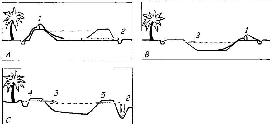
Figure 6: Different types of diversion ponds (Viveen et al., 1985) A: embankment pond B: excavated pond; C: partially excavated pond. See Appendix 1 for an example of how to construct a diversion pond.
