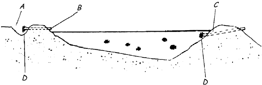
Figure 35: Cross-section of the water inlet and outlet of a pond (Murnyak and Murnyak, 1990). A: silt catchment basin; B: overflow pipe; C: inlet pipe; D: screen.
