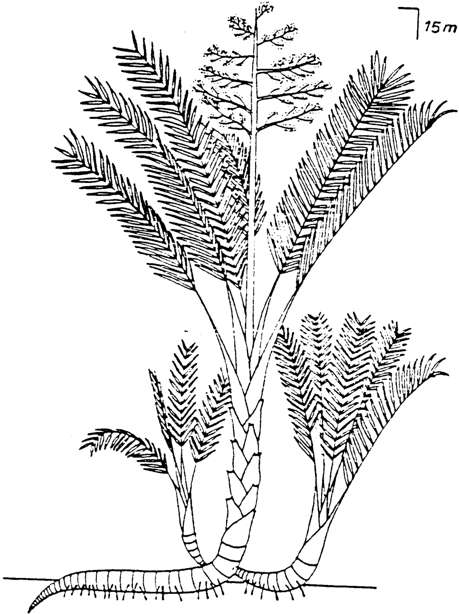
FIGURE 1.—Architecture of Metroxylon sagu , showing hapaxanthic axes. Following Uhl and Dransfield (1987:Figure 5.5).
