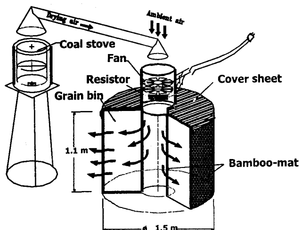
Fig. 1. Construction of SRR-1B dryer with coal stove.
