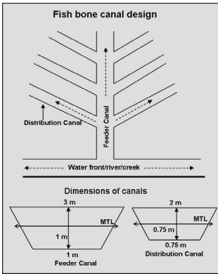
Fig 10.6 Fishbone Canal Design
